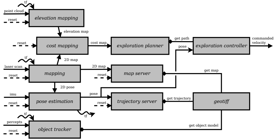
Fig. 2. System overview schematic. ROS nodes are represented by rectangles, topics by arrow-headed and services by diamond-headed lines. Services are originated at the service caller.
